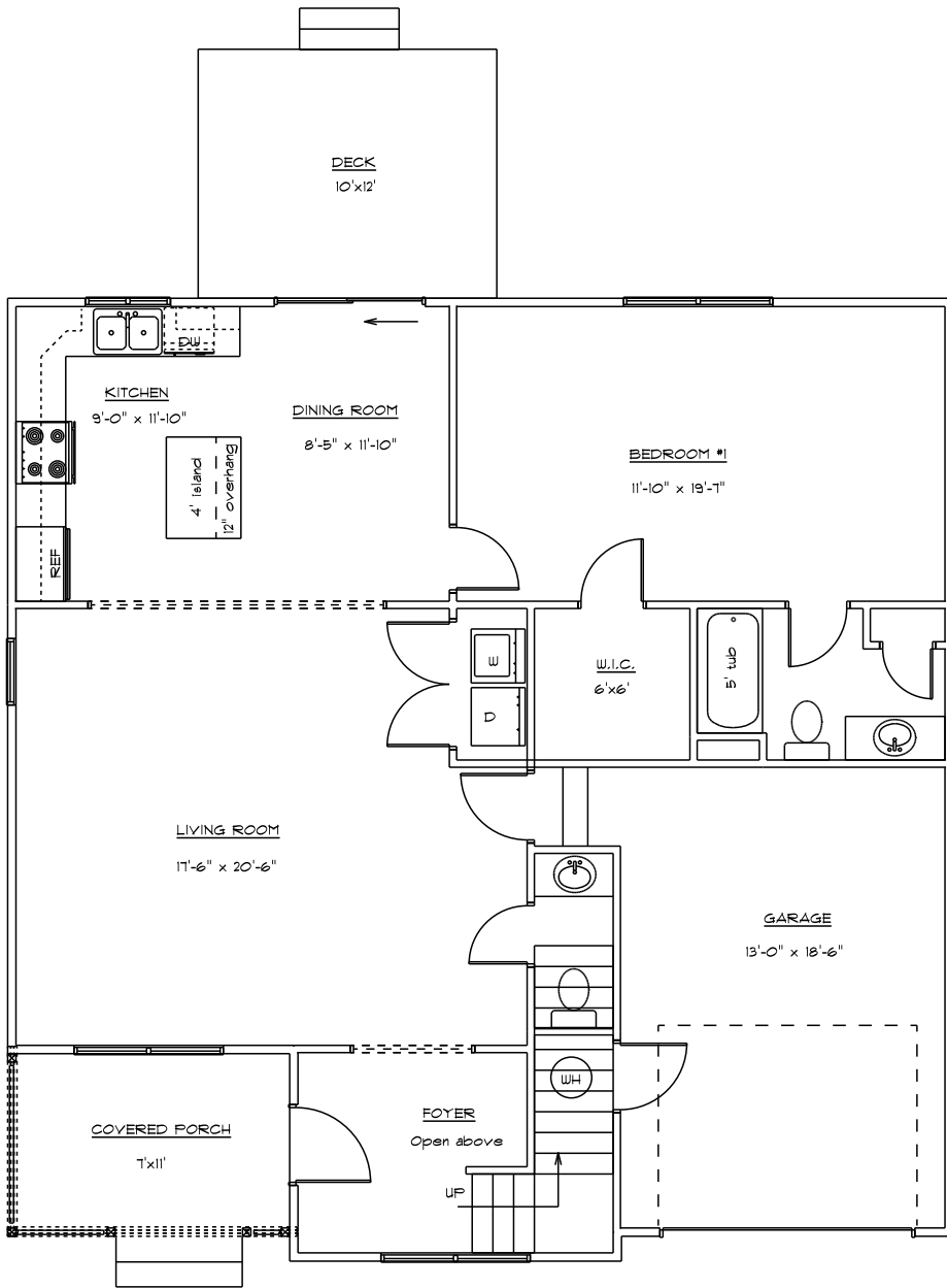
The Winesap Revised First Floor Plan (left unit shown)
