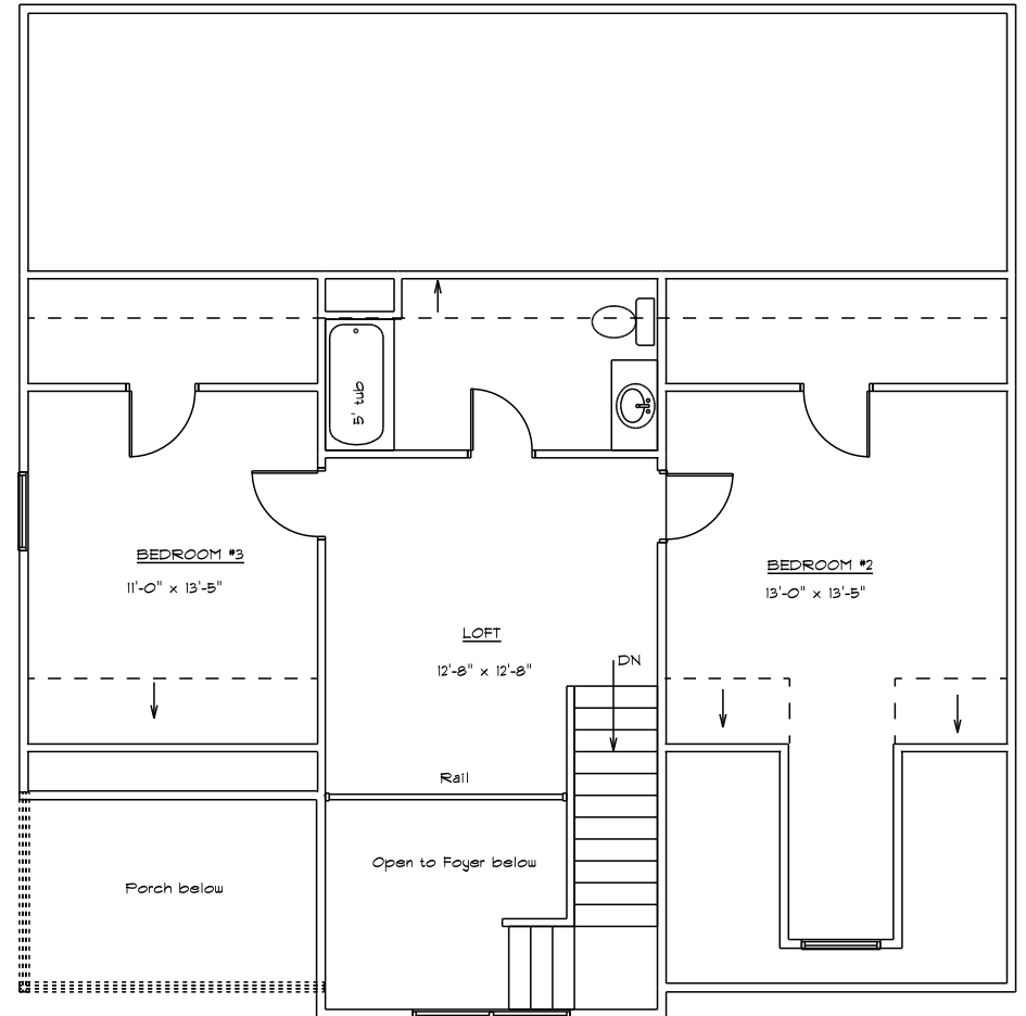
The Winesap Revised Second Floor Plan (left unit shown)
